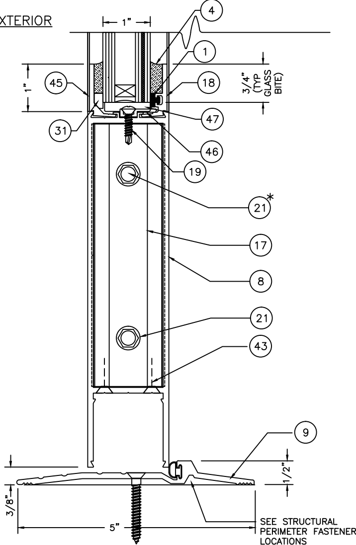
GLAZING DETAIL – BOTTOM RAIL
