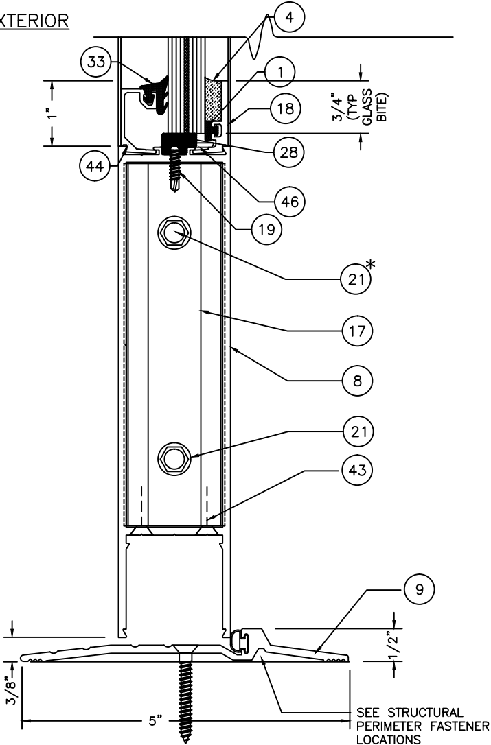
GLAZING DETAIL – BOTTOM RAIL
